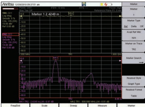
Distance Domain (DTF) analysis allows simultaneous viewing of cable return loss and distance to fault.
